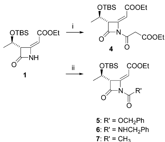
Scheme 5. Reagents: (i) ethyl malonyl chloride, benzene reflux; (ii) K 2 CO 3 , acetone and: CbzCl for 5 , benzyl isocyanate for 6 , and Ac 2 O for 7 .
