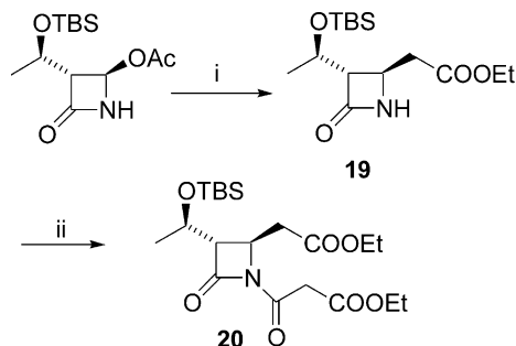
Scheme 6. Reagents: (i) Zn, THF, BrCH 2 COOEt, reflux; (ii) ethyl malonyl chloride, benzene reflux.
