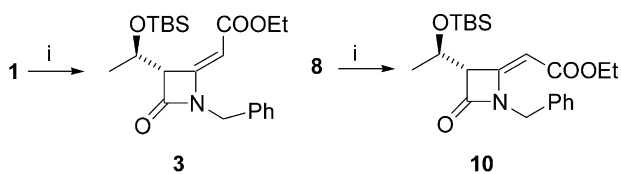
Scheme 4. Reagents: (i) BnBr, K 2 CO 3 , acetone.
