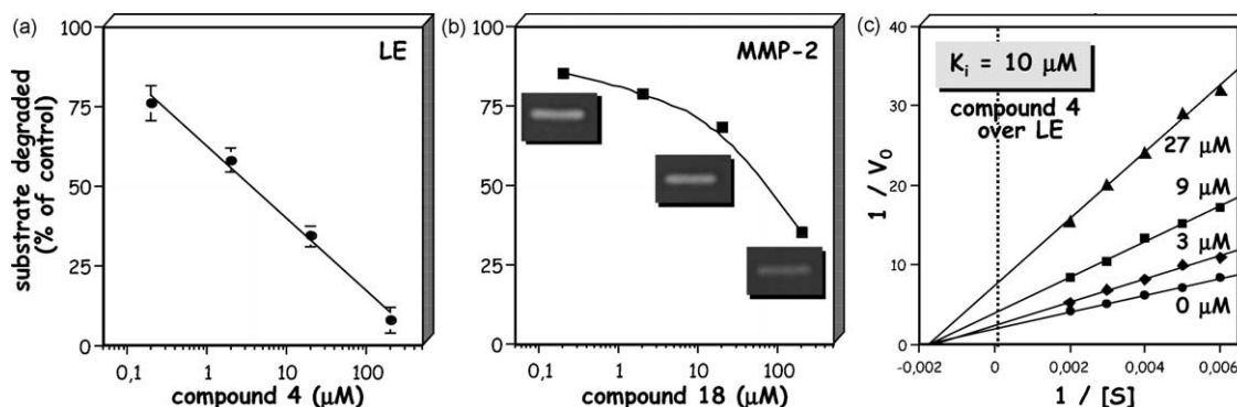
Figure 1. Inhibition of LE and metallo-proteinase-2 (MMP-2) by \beta -lactams 4 and 18 . In the first case (a) a chromogenic substrate (0.4 mM) was incubated at 37 °C with HLE (5 mU) in the presence of increasing concentration of compound 4 (the most efficacious against LE), and the absorbance monitored at 405 nm (values at 60 min are plotted). Each point represents the mean of three digestions. In the second case (b) MMP-2-containing medium was electrophoresed in gelatin-SDS-PAGE, and the zymography developed overnight in the presence of increasing amount of compound 18 (the most efficacious against MMP-2). The MMP-2 digestion bands (inserts) were quantitated by densitometry. Example of duplicate experiment: double-reciprocal plot (c) demonstrating noncompetitive inhibition of LE (5 mU) by increasing concentration of compound 4 ( S = substrate). The points represent the mean values of triplicate samples, with SD < 10%.
