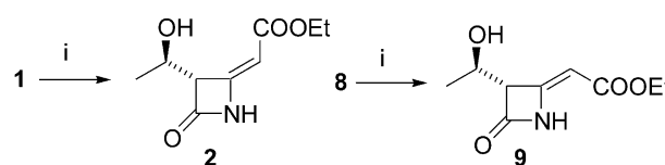
Scheme 3. Reagents: (i) HCl 1 M, \text{CH}_3\text{CN} .
